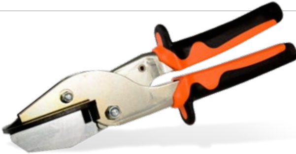
Ref.: 071155 STAINLESS STEEL BLADE 65 MM Re-sharpenable single-block blade.
